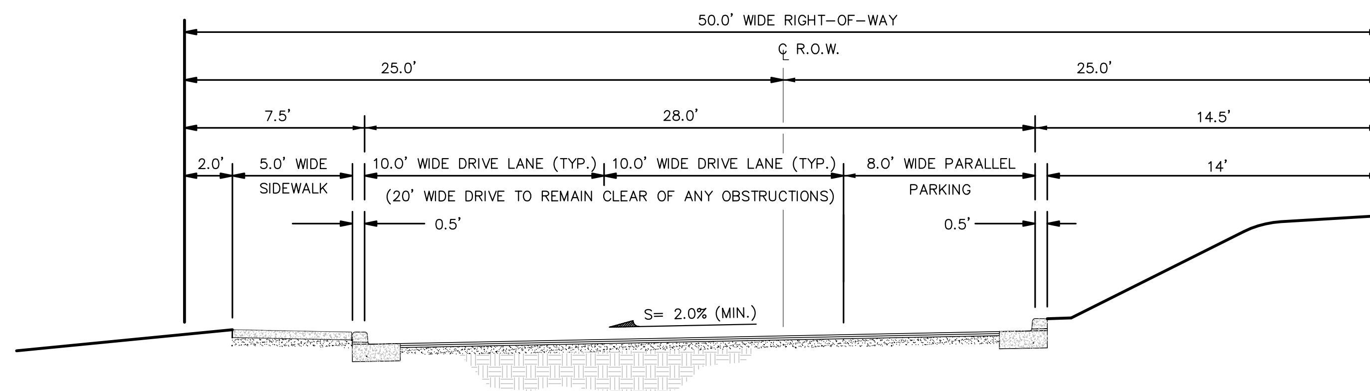
ROAD 'B' CROSS-SECTION
