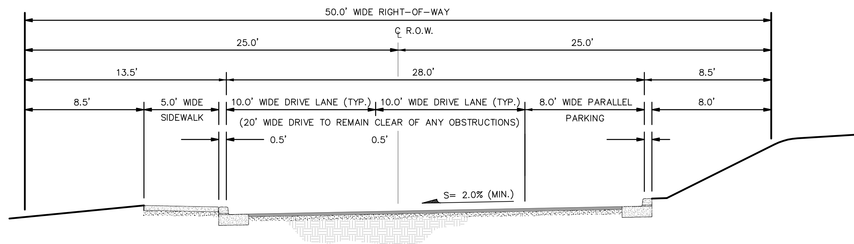
ROAD 'A' CROSS-SECTION
