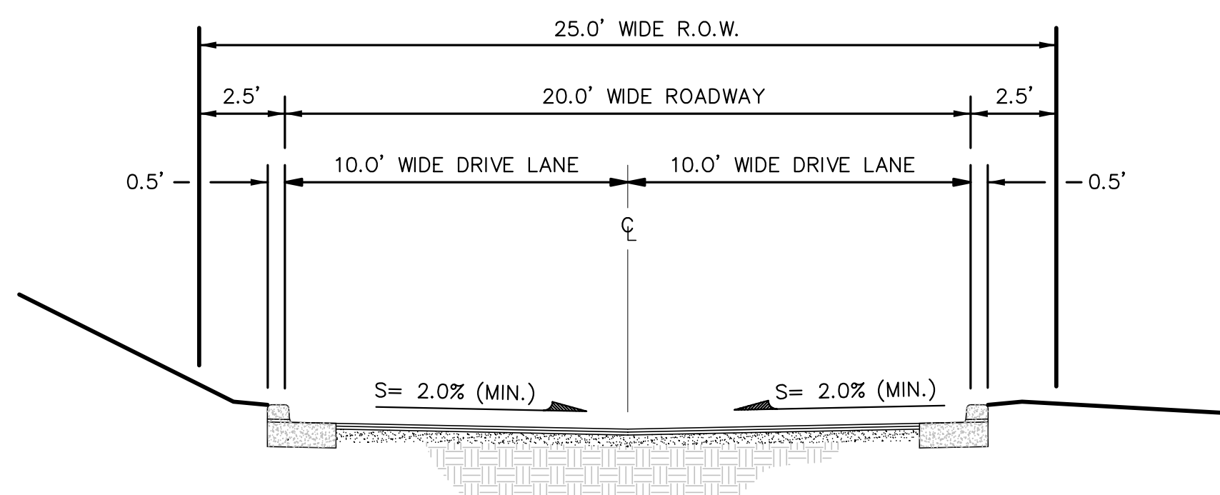
ROAD 'C' CROSS-SECTION
