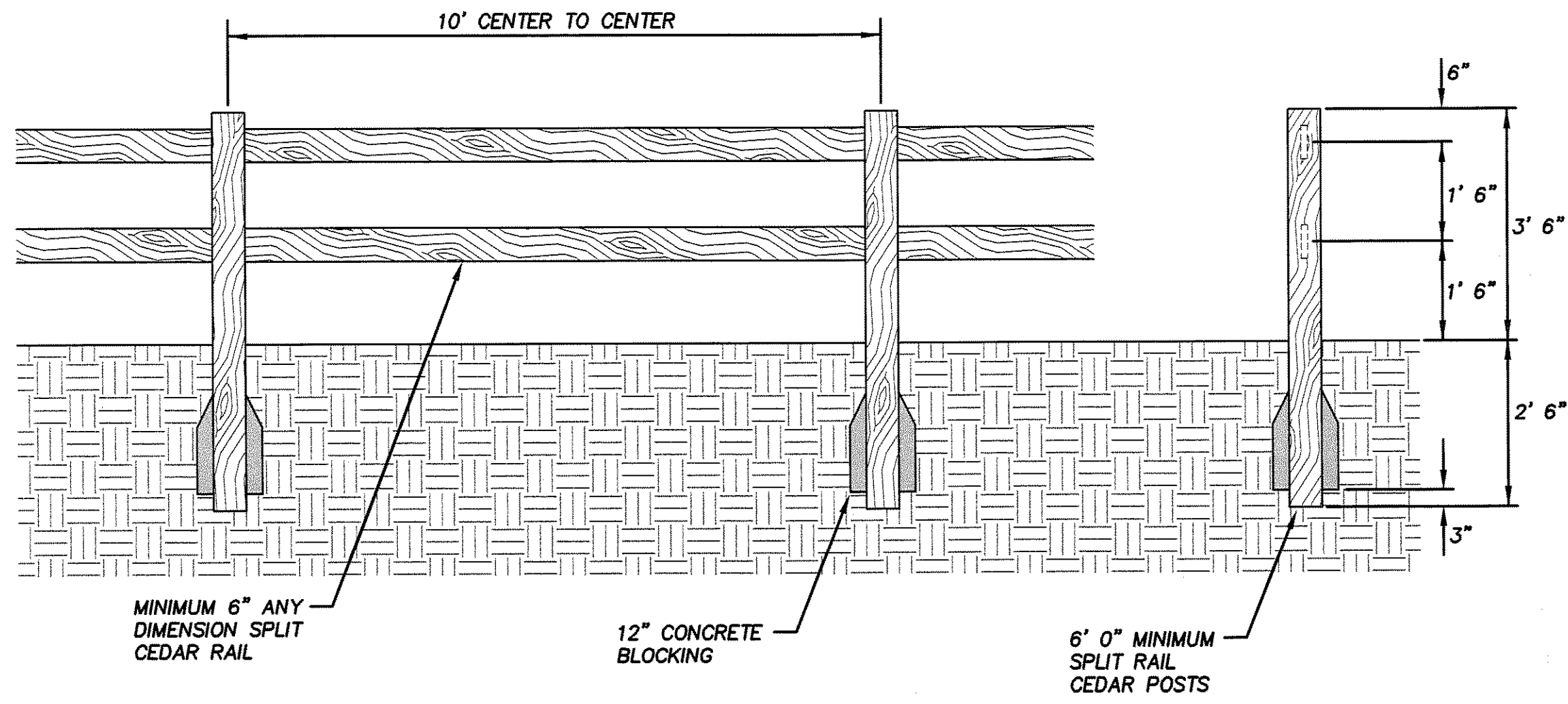
SPLIT RAIL FENCE DETAIL N.T.S.
